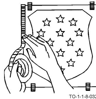
Figure 7-4. Applying Large Emblems (Step 2)
