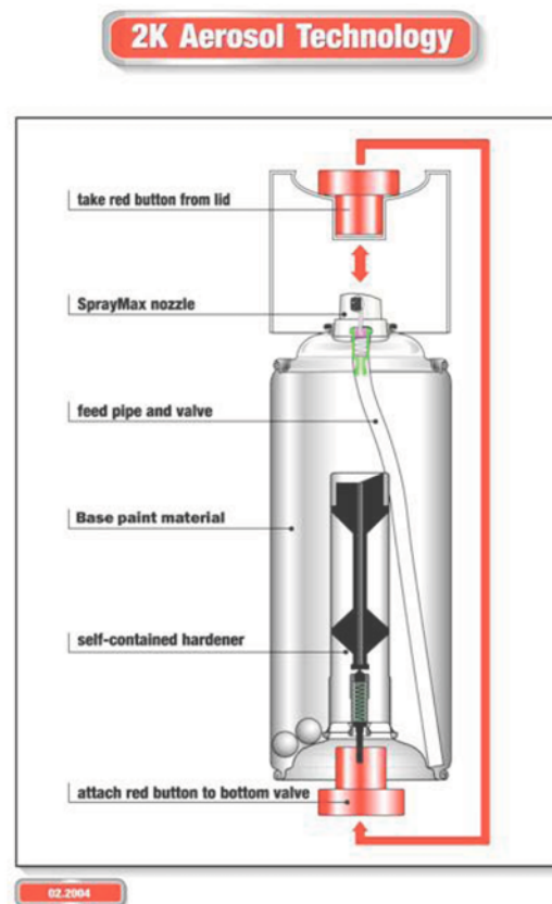
Figure 5-5. Two-Component Aerosol
