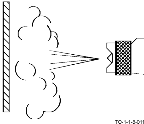
Figure 4-11. Excessive Spray Fog
